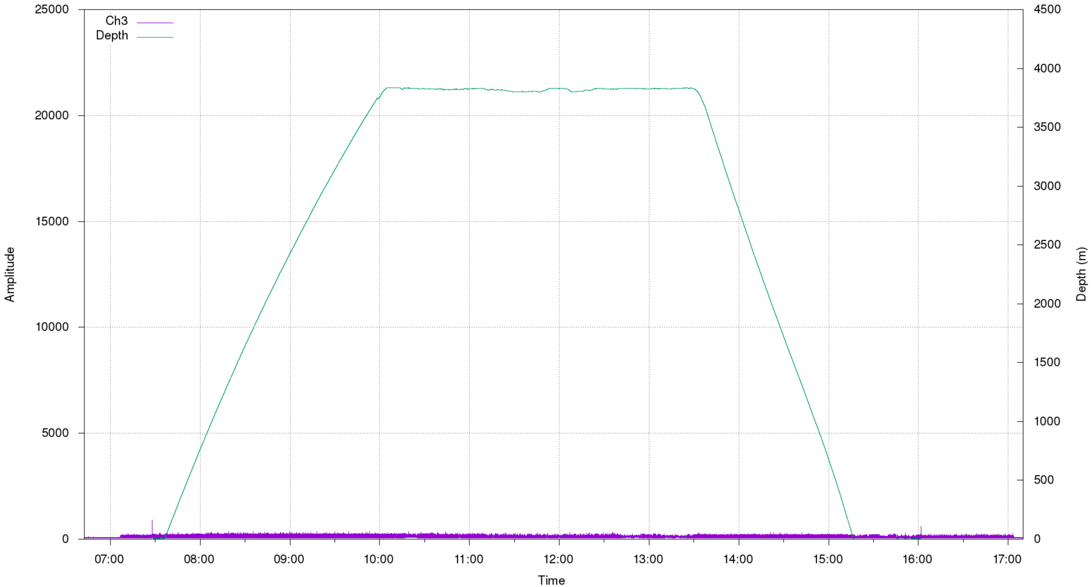
AE Max Amplitude 071522021236 | Ch3
