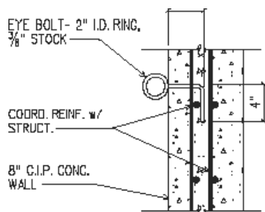
Alternate Weapons Rack Anchor
