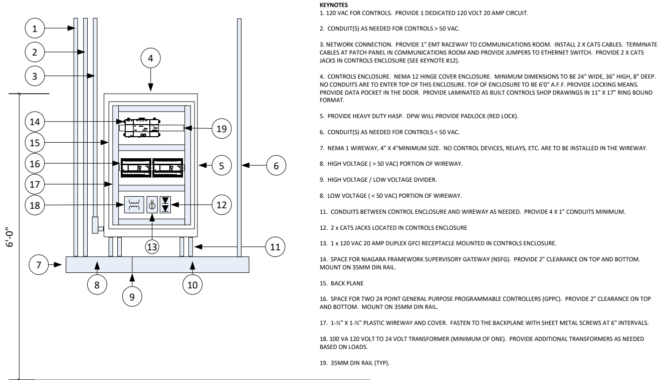
Figure 3– DDC Control Panel Requirements
