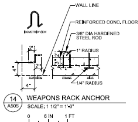
Alternate Weapons Rack Anchor
