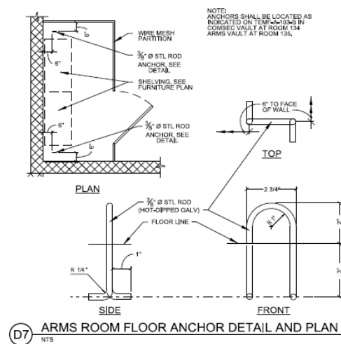
Alternate Weapons Rack Anchor
