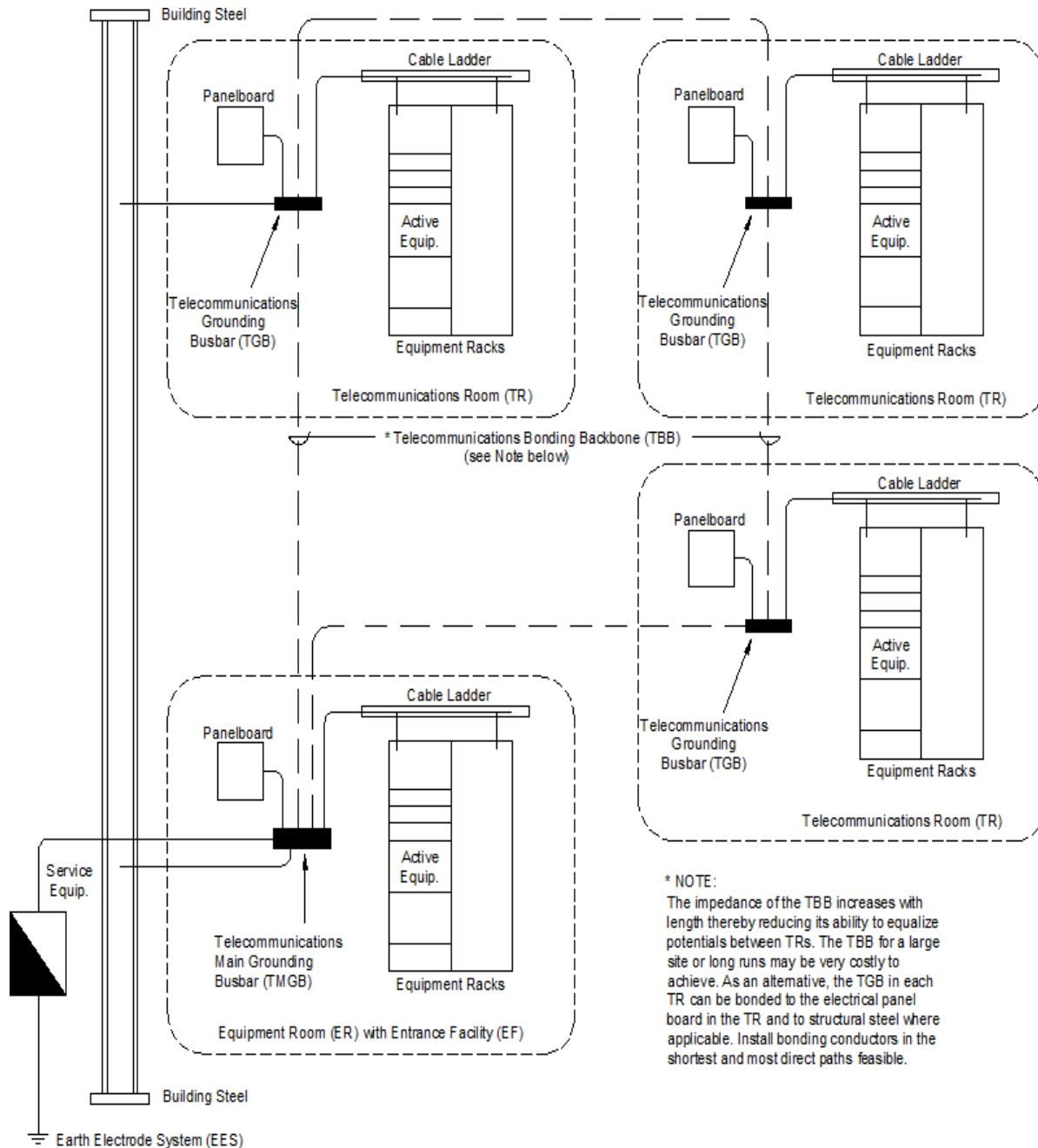
Figure 2-4 – Telecommunications Grounding and Bonding Infrastructure
