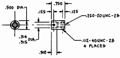
(25) MOTOR/ARM ADAPTOR
