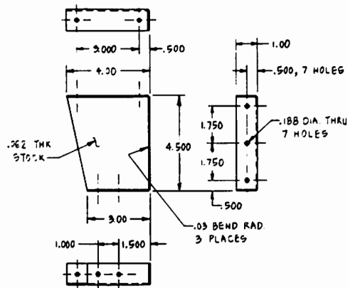
(-17) VERTICAL SUPPORT (FEEDER) SCALE: \frac{1}{2}
