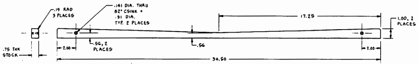
(-41) CONTOUR EDGING, TAPERED
