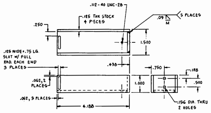
(22) FEEDER
