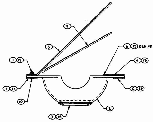
① PIGEON CARRIER ASSEMBLY
