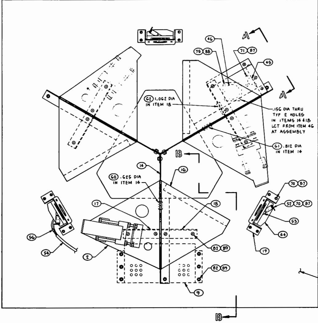
(-1) FLIGHT CONTAINER ASSEMBLY
