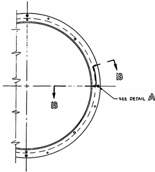
6 VIEWING WINDOW ASSEMBLY SCALE: 1/2
