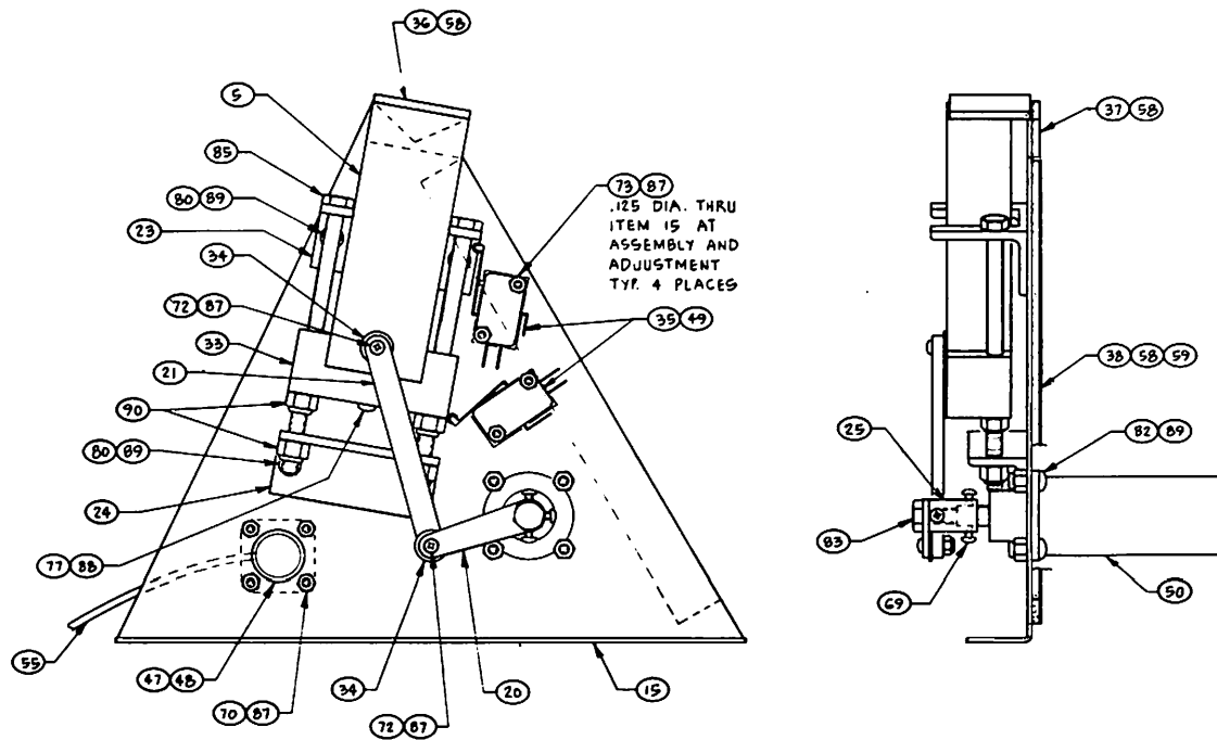
(2) FEEDER SUPPORT PLATE ASSEMBLY
