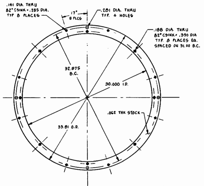
(26) WINDOW FRAME - TOP
