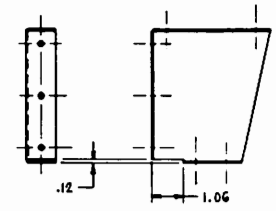
(-18) VERTICAL SUPPORT OTHERWISE OPPOSITE OF ITEM 17 SCALE: \frac{1}{2}
