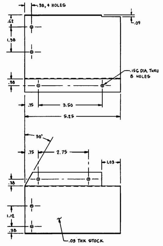
(-11) CONNECTOR COVER
