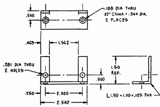
(23) FEEDER MOUNT/GUIDE
