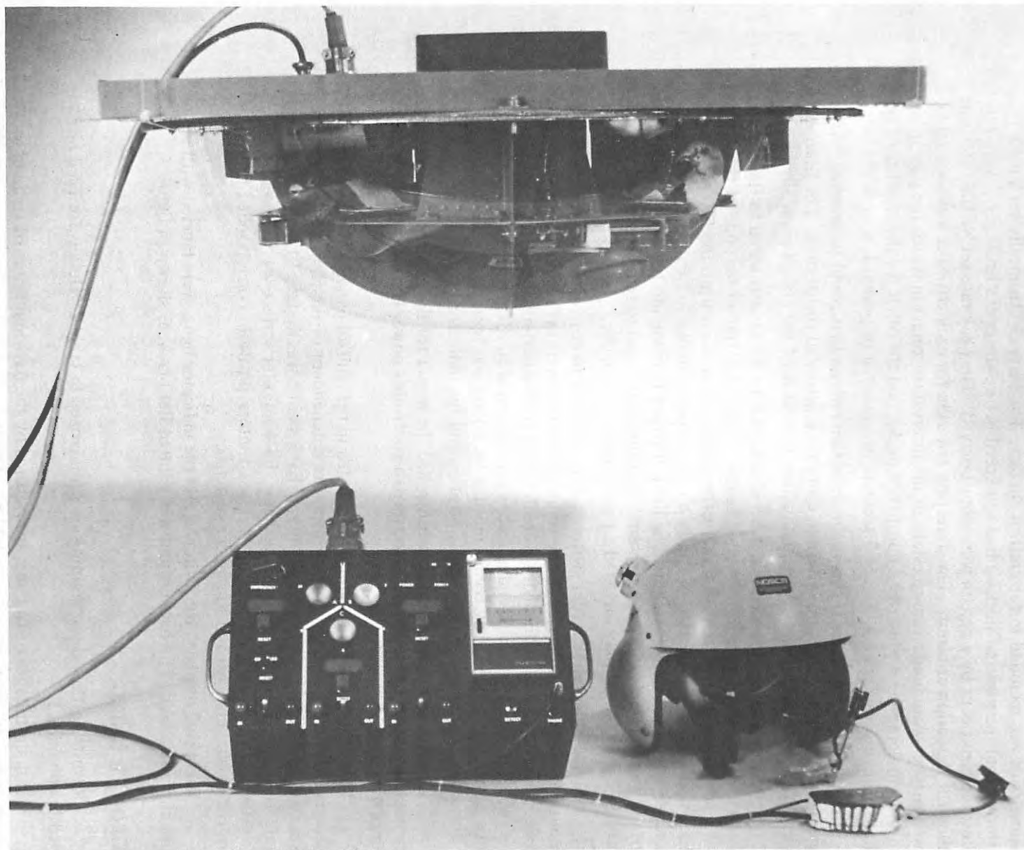
Figure 3. Flight equipment: observation container with pigeons (top); control/display panel (lower left); and crew member's helmet (lower right).
