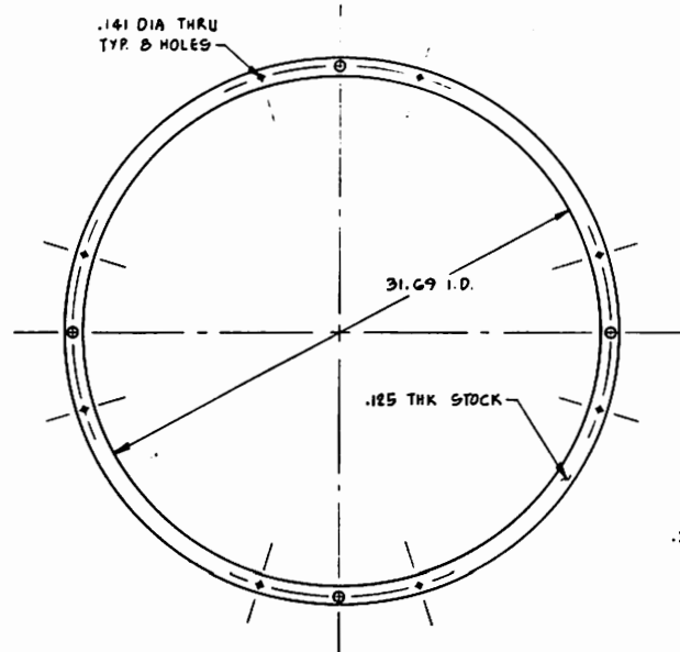
(-28) WINDOW FRAME - CENTER OTHERWISE SHAPE AND HOLE LOCATION SAME AS ITEM 26 SCALE: \frac{1}{4}
