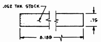
(-3) PADDING, OPENING
