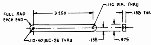
(21) EXTENSION ARM
