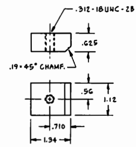
(-30) MOUNT, REAR, STATIONARY SCALE: \frac{1}{1}
