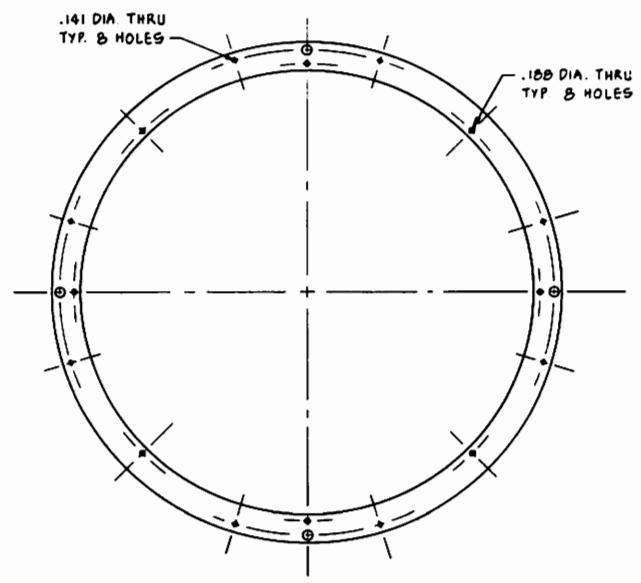
(27) WINDOW FRAME - BOTTOM OTHERWISE SHAPE AND HOLE LOCATION SAME AS ITEM 26
