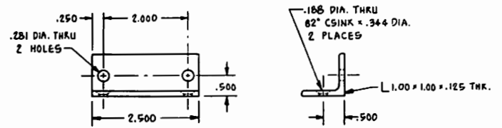
(24) FEEDER MOUNT
