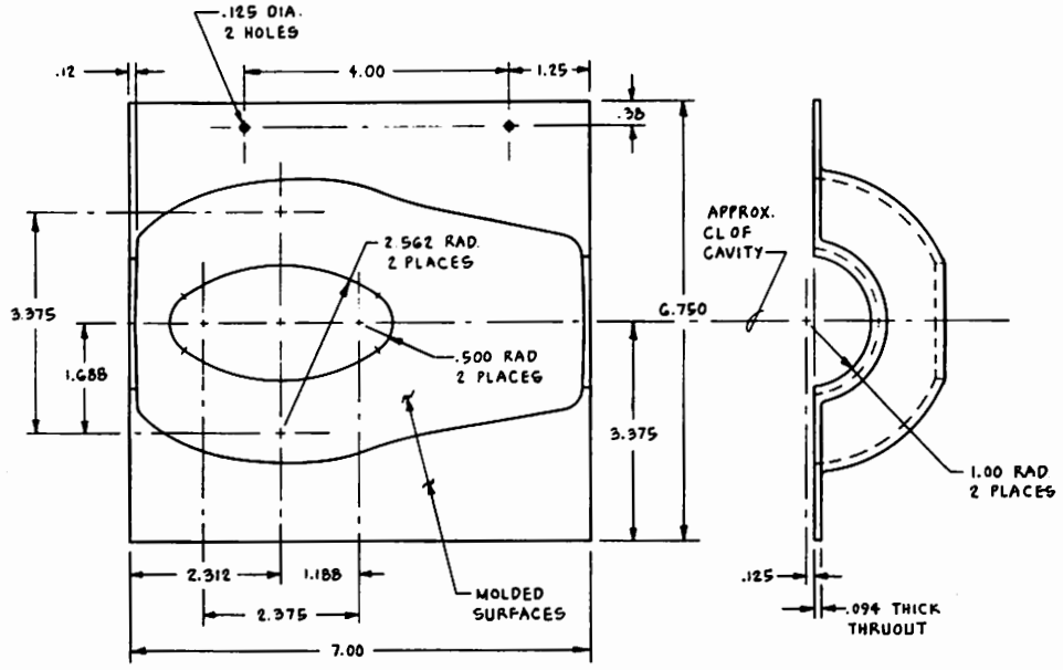
(-2) CARRIER
