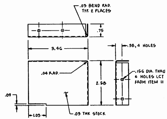
(-10) CONNECTOR COVER END PLATE
