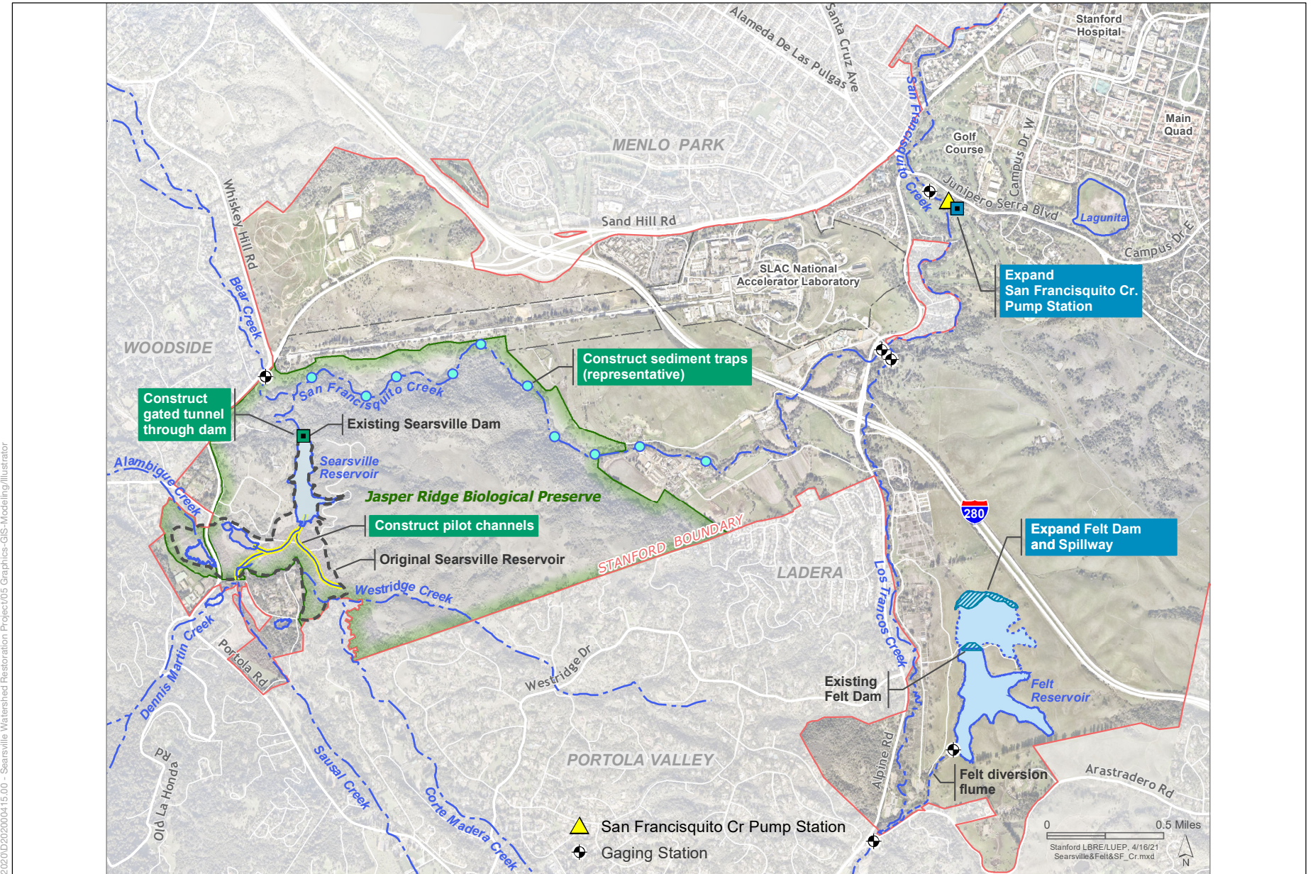
Figure 2 Proposed construction components
