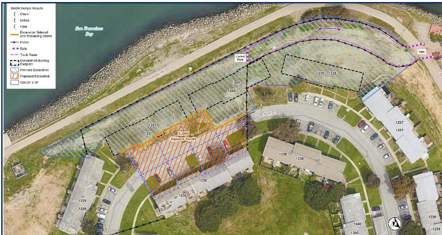
- NTCRA Excavation Layout
