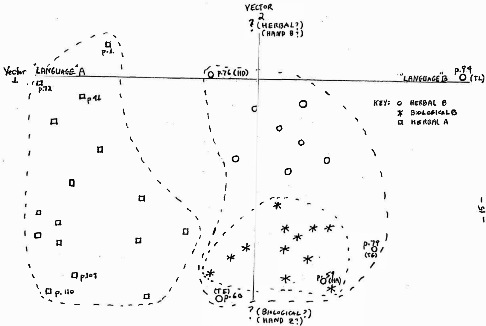
Results of Minissa (Multidimensional scaling) Program
