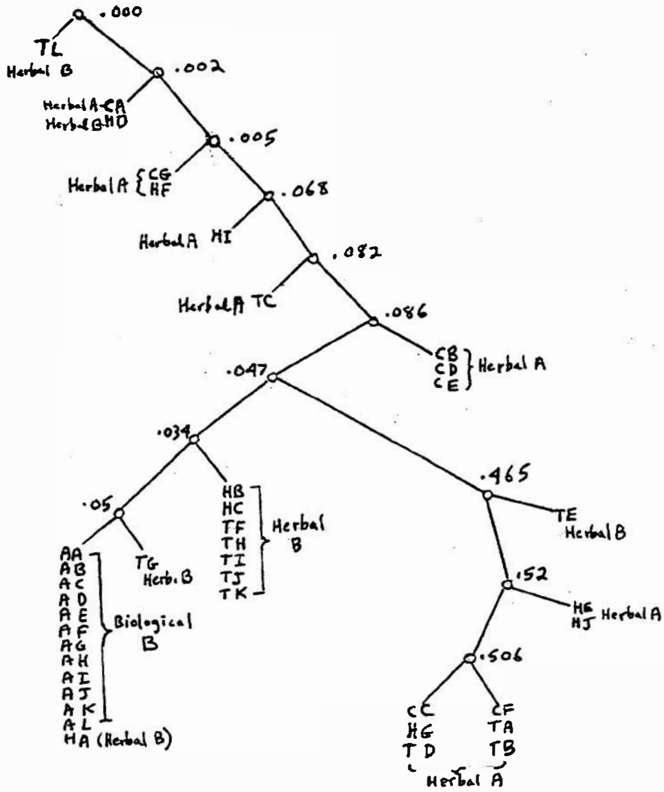
PEP-1 "Family Tree" (Single Linkage Clusters)
