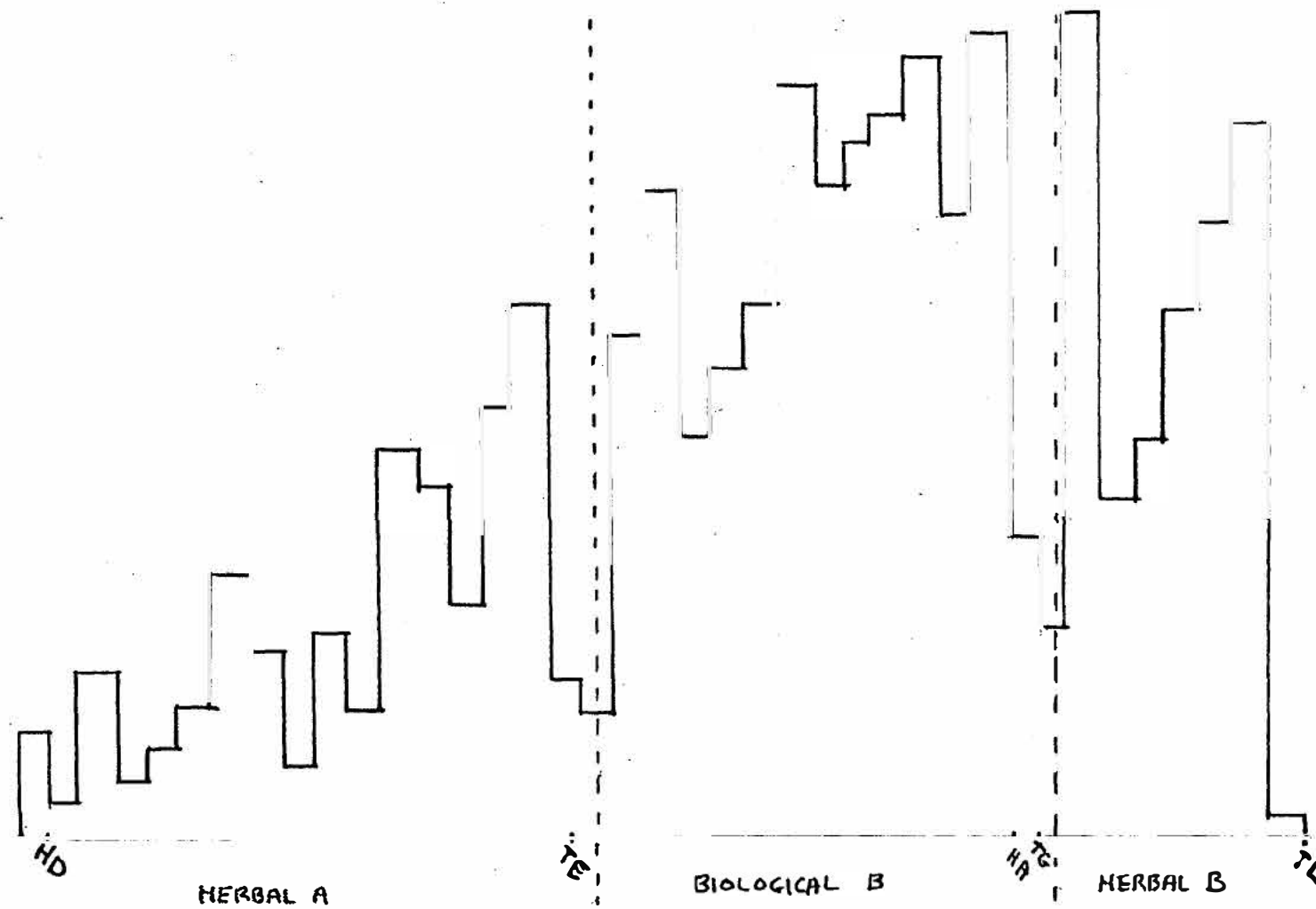
RESULTS OF MICLUS Figure 4
