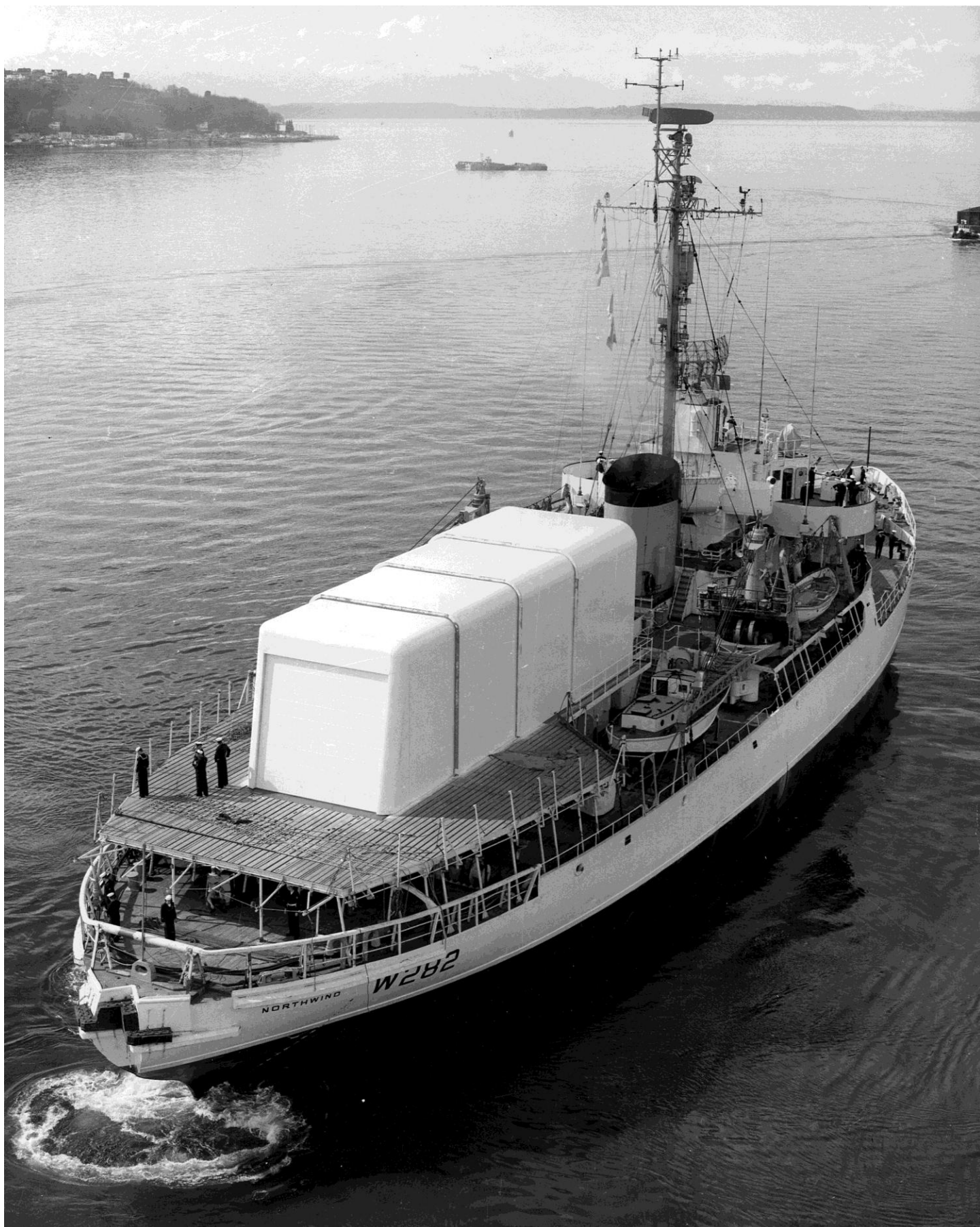
USCGC Northwind with a retractable helicopter hangar, 1963.
