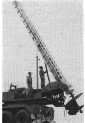
BIG BORE—Army's new earth auger can dig holes with record-breaking speed for storage and waste disposal.
