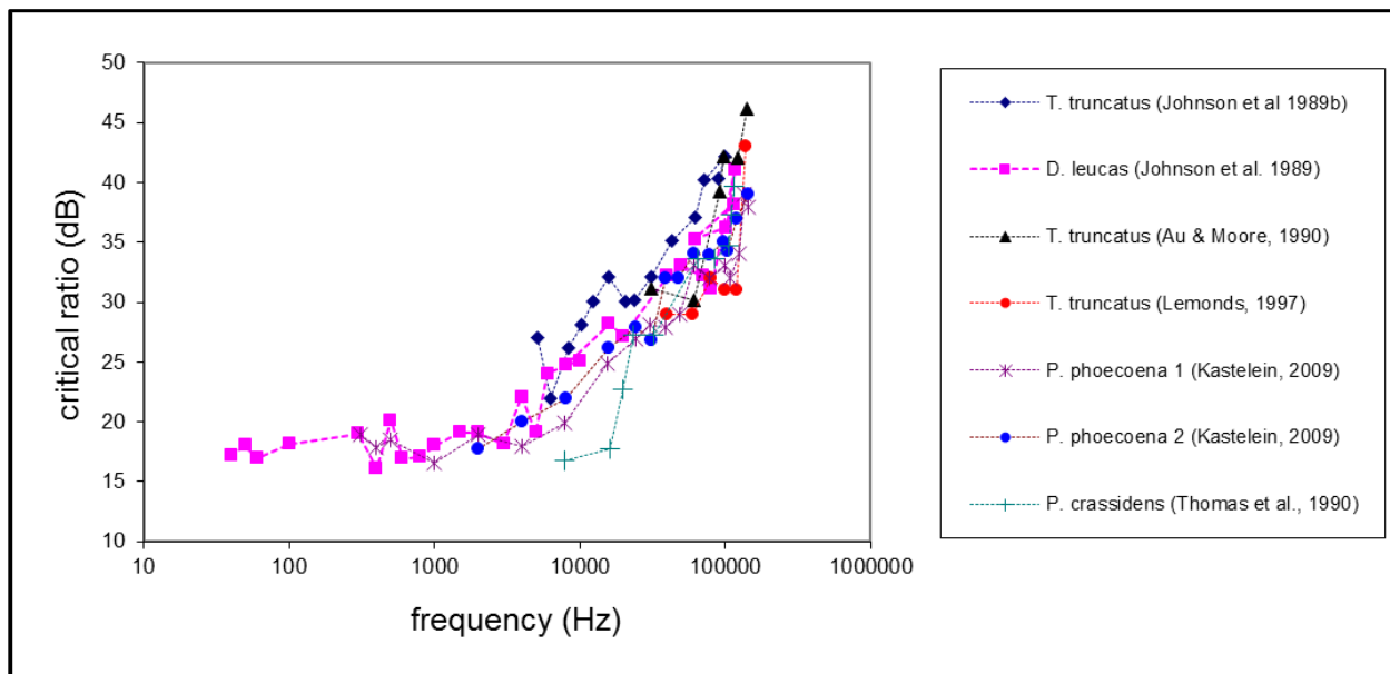
Figure 3.7-5: Critical Ratios (in dB) Measured in Different Odontocetes Species (from Finneran & Branstetter, 2013)
