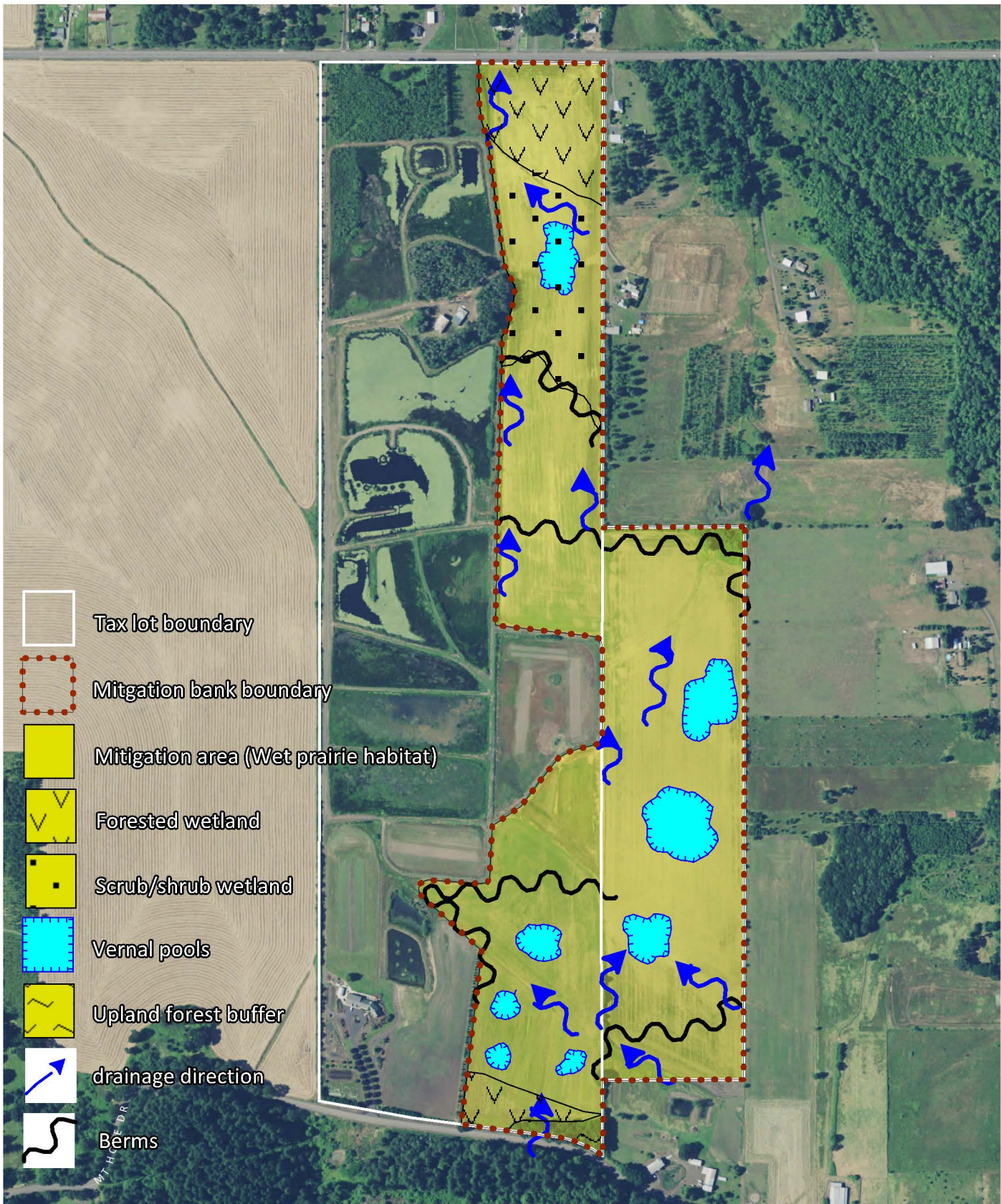
FIGURE 4: MITIGATION SITE PLAN
