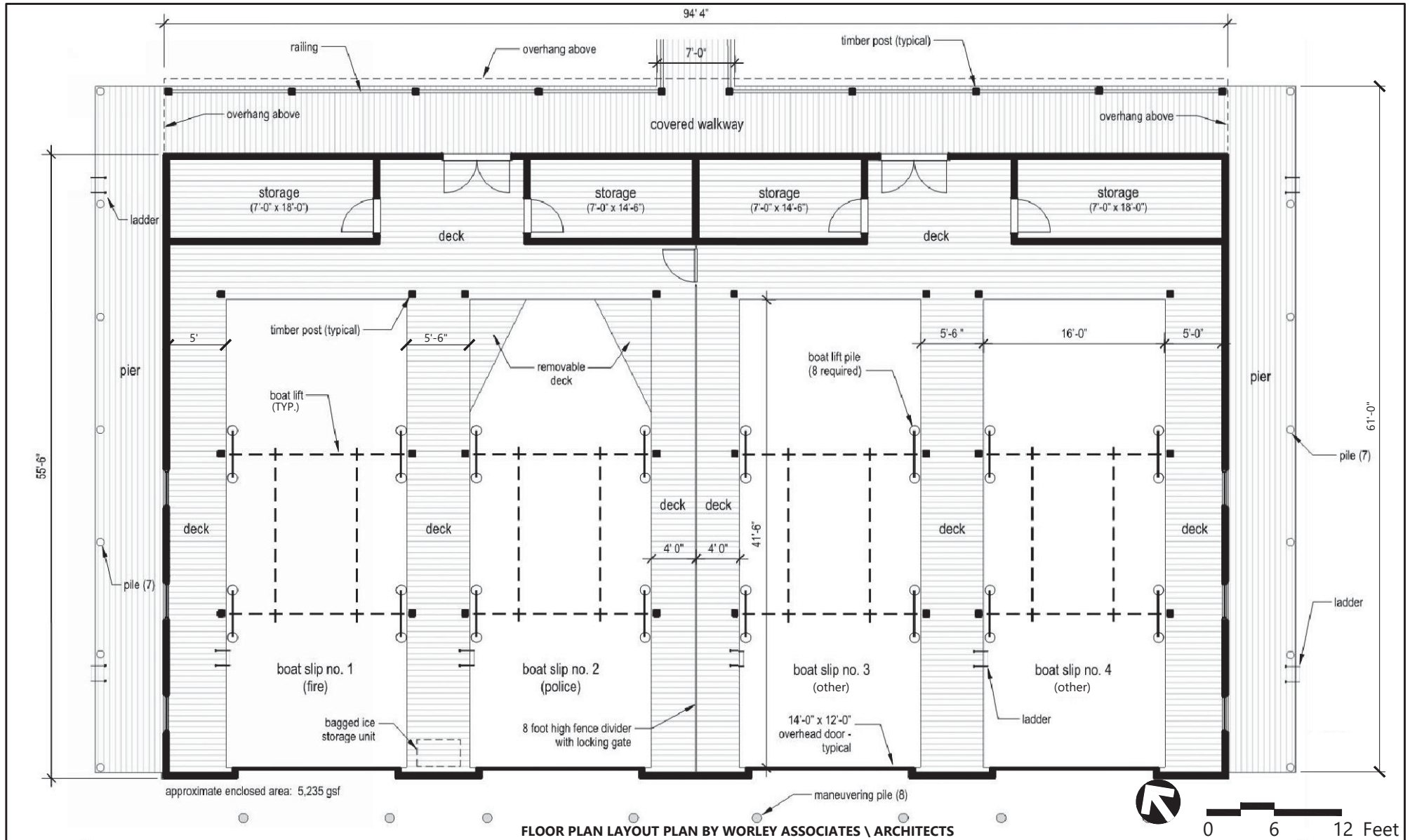
FLOOR PLAN LAYOUT PLAN BY WORLEY ASSOCIATES \ ARCHITECTS
