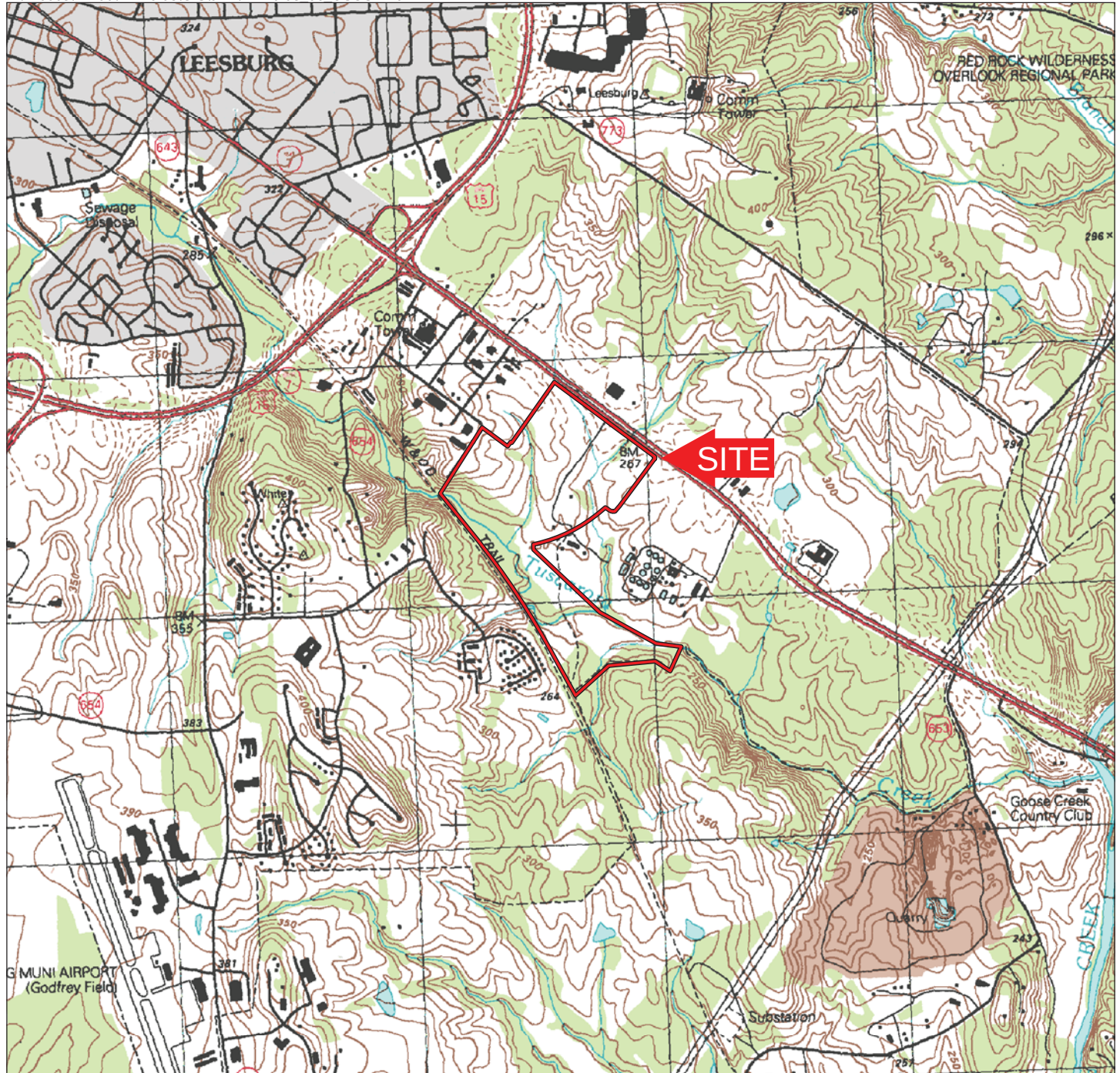
USGS Quad Map Leesburg, VA-MD 1994 Leegate WSSI #21479.03 Original Scale: 1" = 2000'
