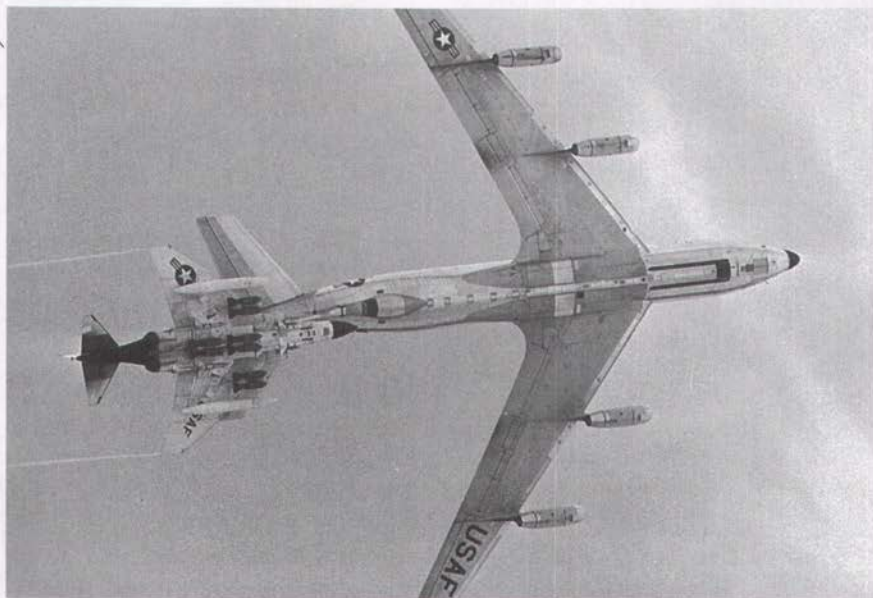
The lights that guide a pilot into the proper position for refueling appear as small squares on the fuselage just behind the wing on this KC-135.
