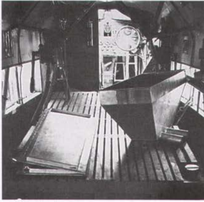
The cabins of the receiver (left) and the tanker. In the receiver, the fueling hose was placed in the funnel, which fed the cabin tanks under the duck boards at center. The tanker's refueling system has three gate valves, a levered quick closing valve, and a strainer in front of the hose.
