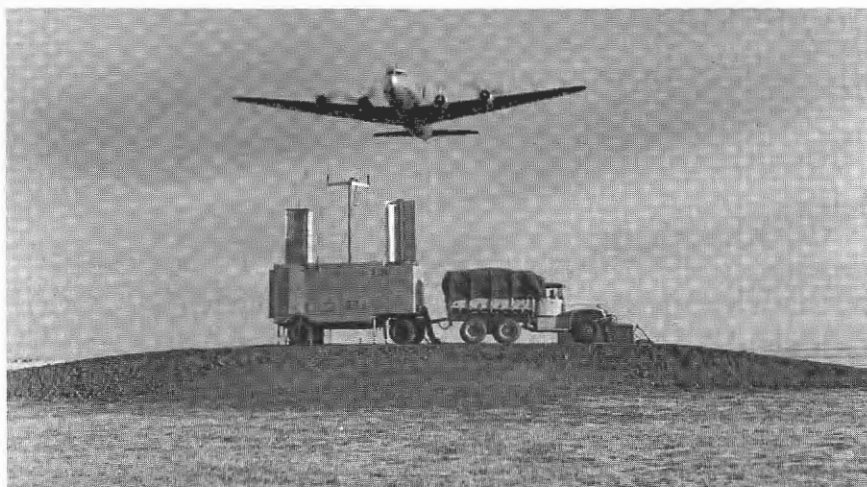
"The need for additional pilots, aircrew, and maintenance personnel." A Douglas C-54 Skymaster comes in low over the GCA van at the Replacement Training Unit at Great Falls Air Force Base, Montana. (U.S. Air Force.)
