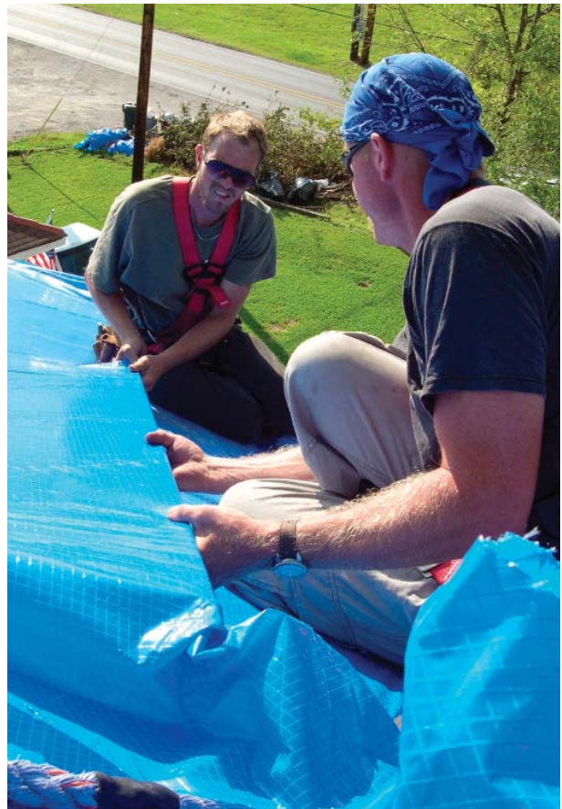
Corps of Engineers contractors install a blue roof on a house in eastern Jefferson Parish, Louisiana in support of Hurricane Katrina recovery efforts.
